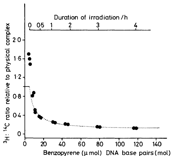
FIGURE 1 3 H: 14 C Ratio (d.p.m.) for benzo[ a ]pyrene covalently bound to native calf thymus DNA by ultraviolet irradiation as a function of irradiation duration (top) and of net binding to DNA (bottom) (calculated on carbon-14 association to DNA). Theoretical curve calculated for 92% loss of tritium from hydrocarbon photochemically bound to DNA and no loss of tritium from 'dark' hydrocarbon-binding.
